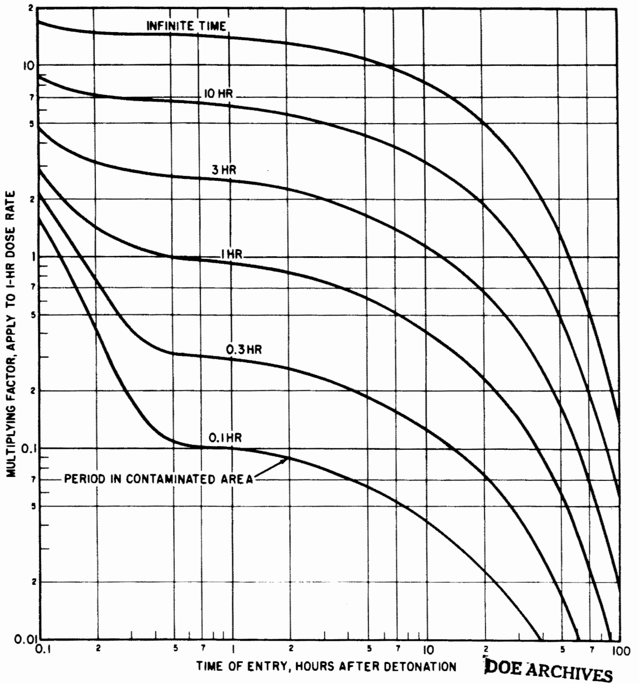
Figure 4-61. Total Radiation Dose Received in an Area Contaminated by Neutron-induced Gamma Activity, Soil Type II
